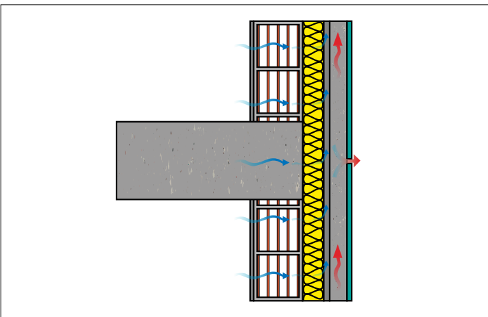
Cessione dell’eccesso di vapore acqueo proveniente dall’interno dell’edificio nell’ambiente esterno. Transfer of the exceeding water vapour from inside the building to the external environment.
